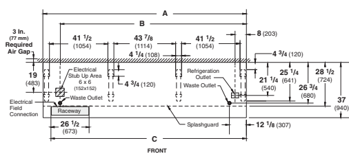
C5NX-LE 4', 6', 8' and 12' Plan Views
