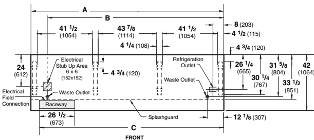
C5X 4', 6', 8' and 12' Plan Views
