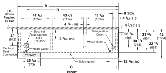
M5X-E, M5X-GE, M5X-EP, M5X-GEP Plan Views
