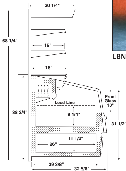
End View With Optional Lighted Superstructure
